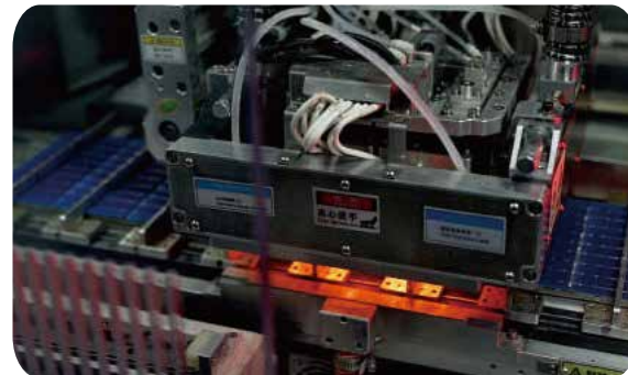
2.AUTOMATIC WELDING
